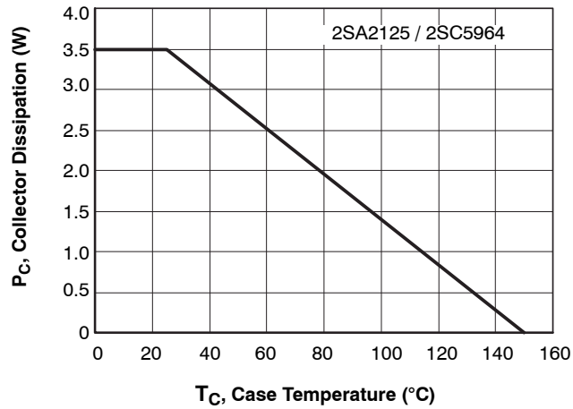
Figure 20. P C - T C
