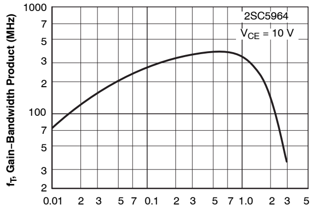
I_C , Collector Current (A) Figure 9. f_T - I_C
