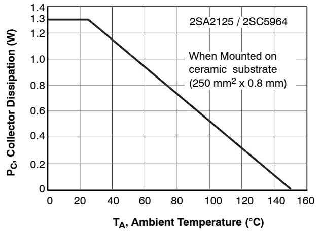
Figure 19. P_C - T_A
