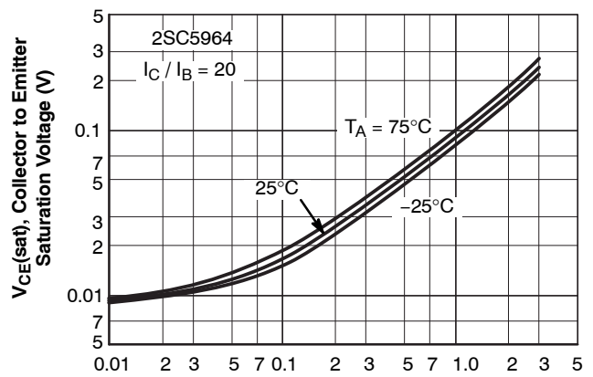
I_C , Collector Current (A) Figure 13. V_{CE(sat)} - I_C
