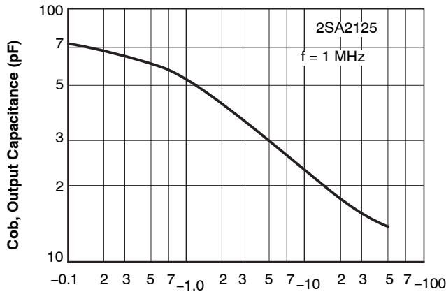
V_{CB} , Collector to Base Voltage (V) Figure 10. C_{ob} - V_{CB}
