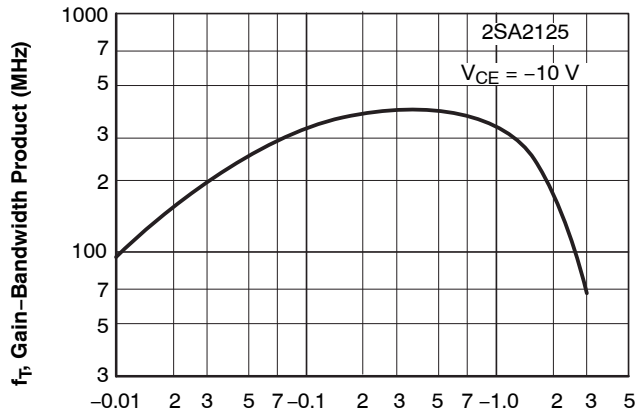
I_C , Collector Current (A) Figure 8. f_T - I_C
