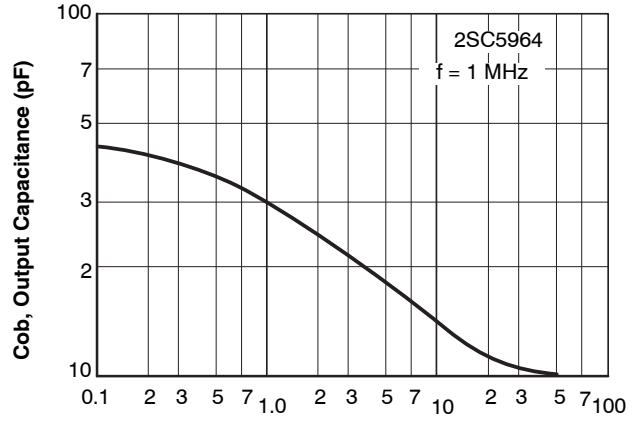
V_{CB} , Collector to Base Voltage (V) Figure 11. C_{ob} - V_{CB}
