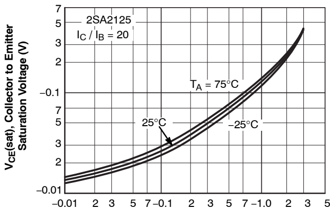
I_C , Collector Current (A) Figure 12. V_{CE(sat)} - I_C
