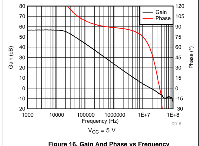
Figure 16. Gain And Phase vs Frequency
