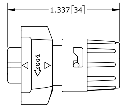
SHOWN ASSEMBLED KIT ASSY: W6382-2SG-P-3XX SHOWN
