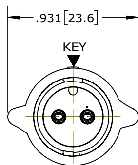
MATING FACE ASSY: W6382-2SG-P-3XX SHOWN
